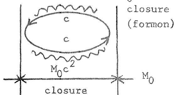
Figure IX-13. Why E=M_0c^2 in a
